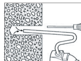
Clean hole and insert anchor with plug inside.
